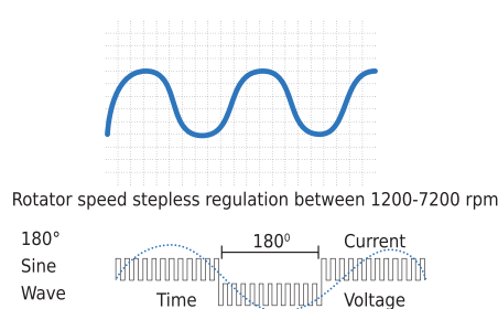
180° Sine Wave D.C. Control
