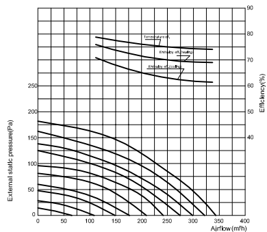
CH-HRV2.5KDC Performance Chart
