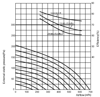
CH-HRV5KDC Performance Chart
