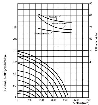
CH-HRV3.5KDC Performance Chart
