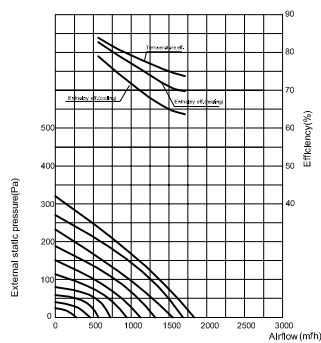
CH-HRV15KDC Performance Chart
