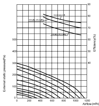
CH-HRV10KDC Performance Chart
