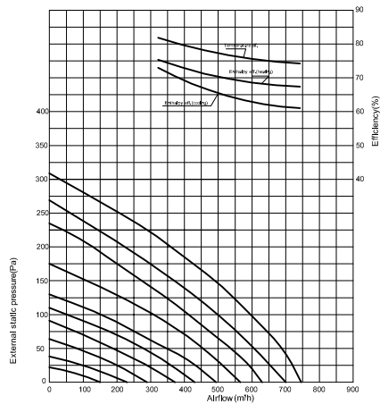
CH-HRV6.5KDC Performance Chart
