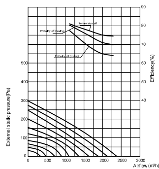
CH-HRV20KDC Performance Chart
