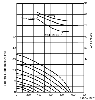
CH-HRV8KDC Performance Chart
